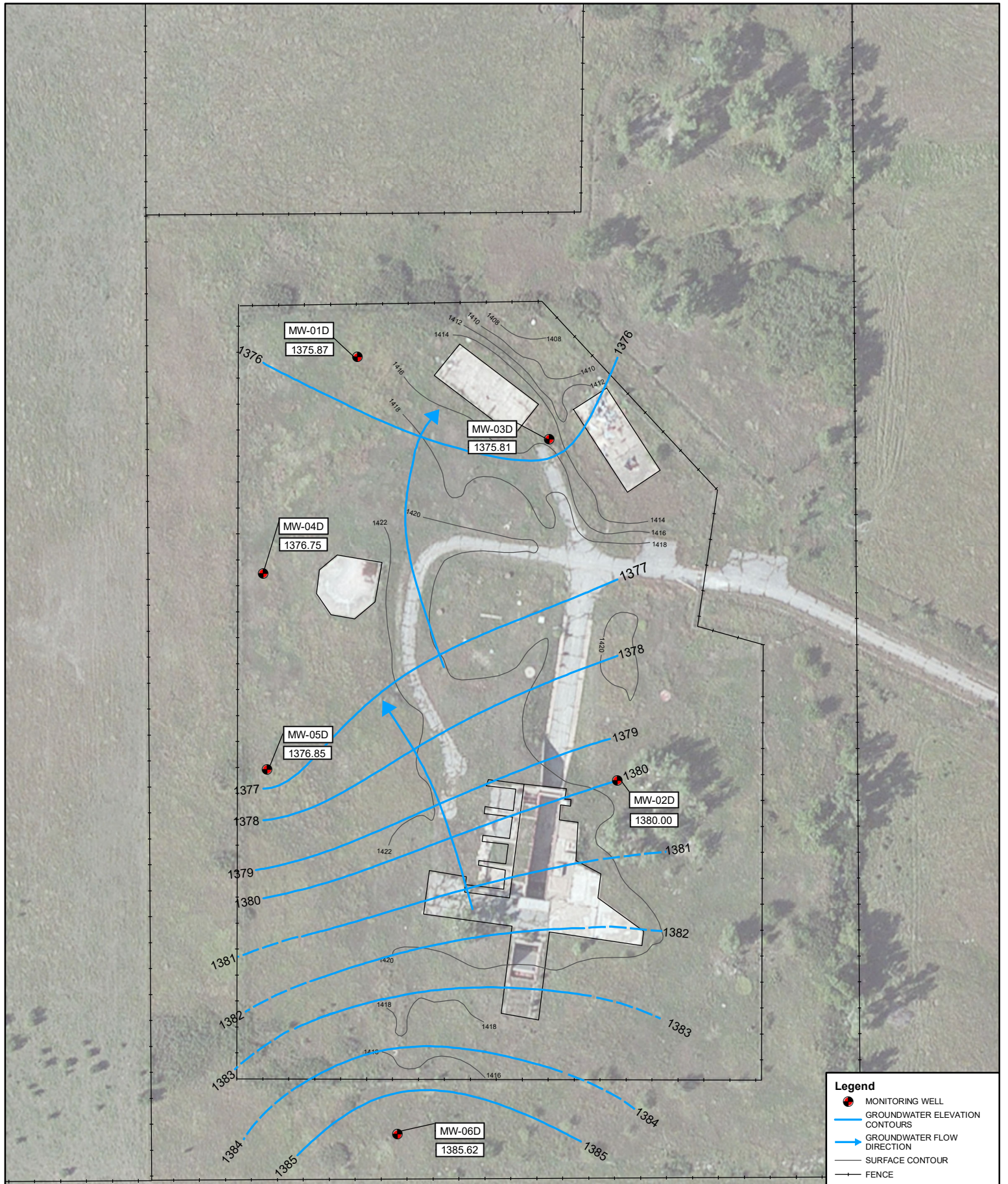
FIGURE 1 GROUNDWATER ELEVATION MAP DEEP MONITORING WELL LOCATIONS FORBES ATLAS S-5 ALLEN, KANSAS DECEMBER 14, 2015
