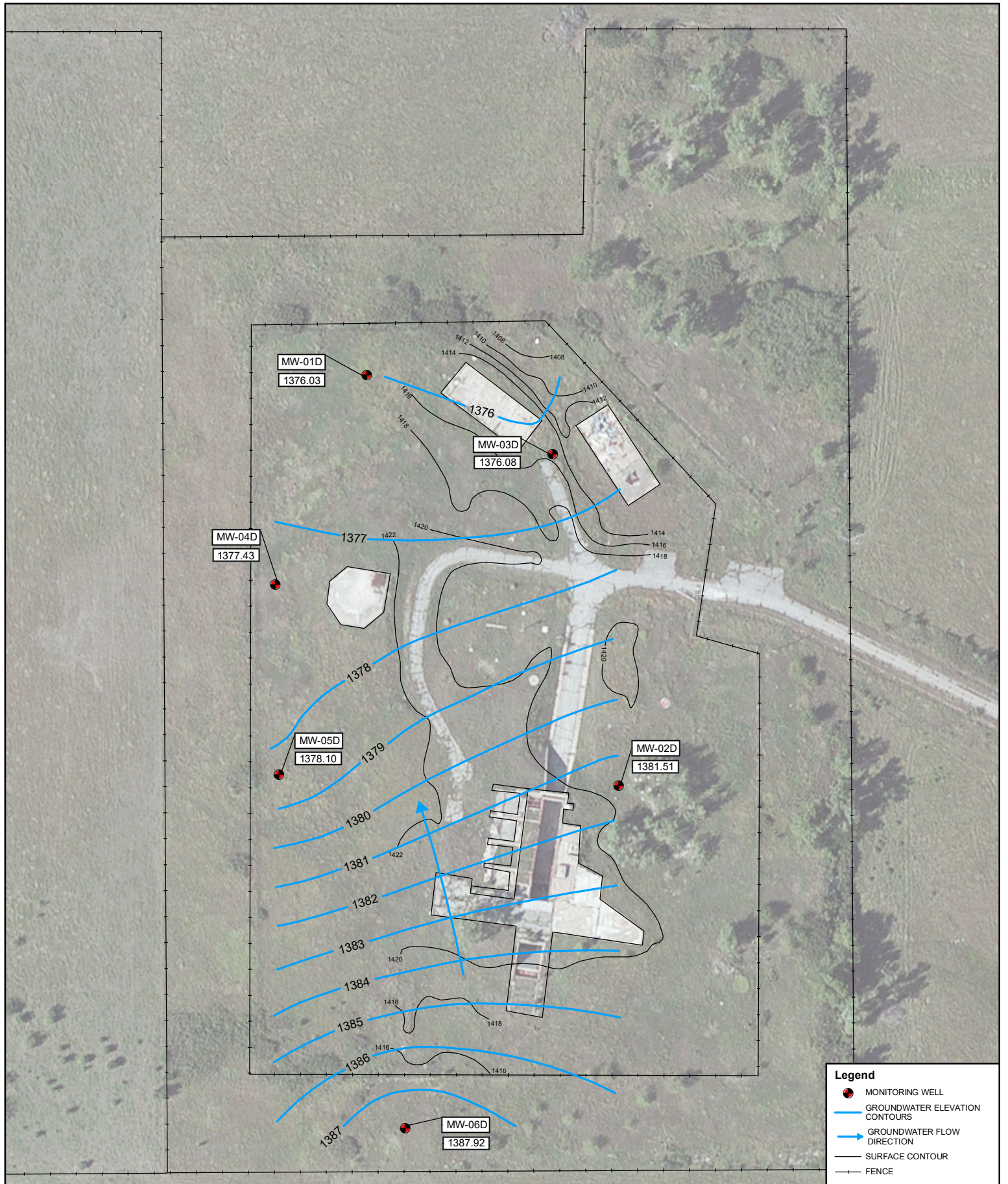
FIGURE 1 GROUNDWATER ELEVATION MAP DEEP MONITORING WELL LOCATIONS FORBES ATLAS S-5 ALLEN, KANSAS JULY 6, 2015
