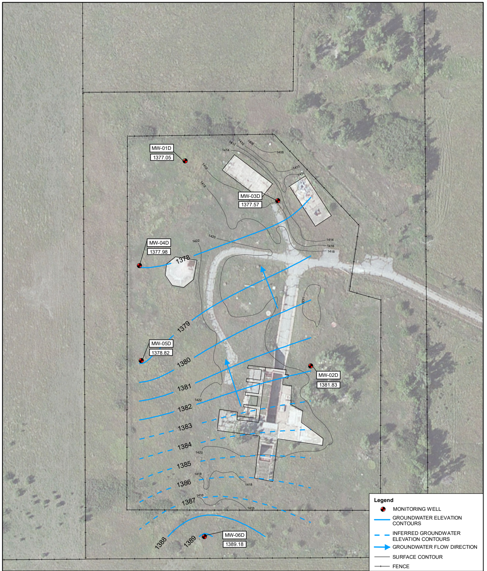
FIGURE 1 GROUNDWATER ELEVATION MAP DEEP MONITORING WELL LOCATIONS FORBES ATLAS S-5 ALLEN, KANSAS MARCH 7, 2016
