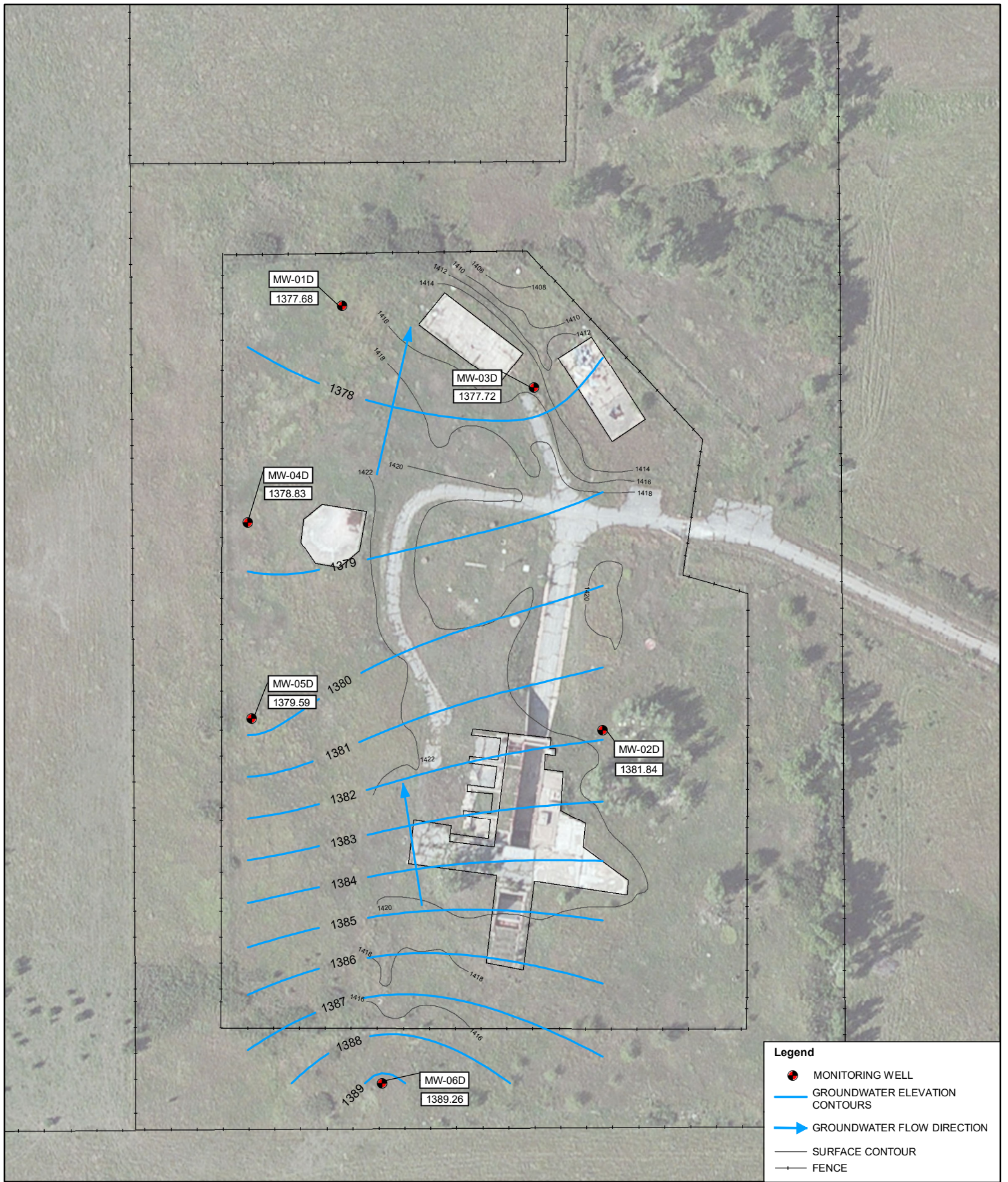
FIGURE 1 GROUNDWATER ELEVATION MAP DEEP MONITORING WELL LOCATIONS FORBES ATLAS S-5 ALLEN, KANSAS MARCH 27, 2017
