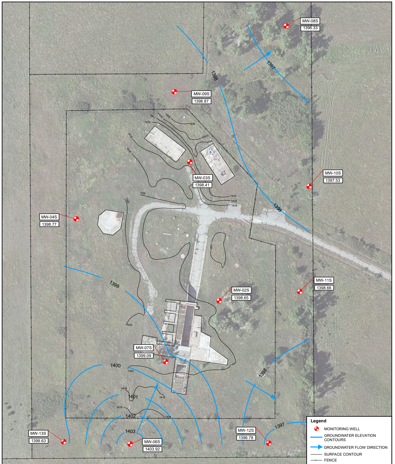
FIGURE 2 GROUNDWATER ELEVATION MAP SHALLOW MONITORING WELL LOCATIONS FORBES ATLAS S-5 ALLEN, KANSAS MARCH 27, 2017
