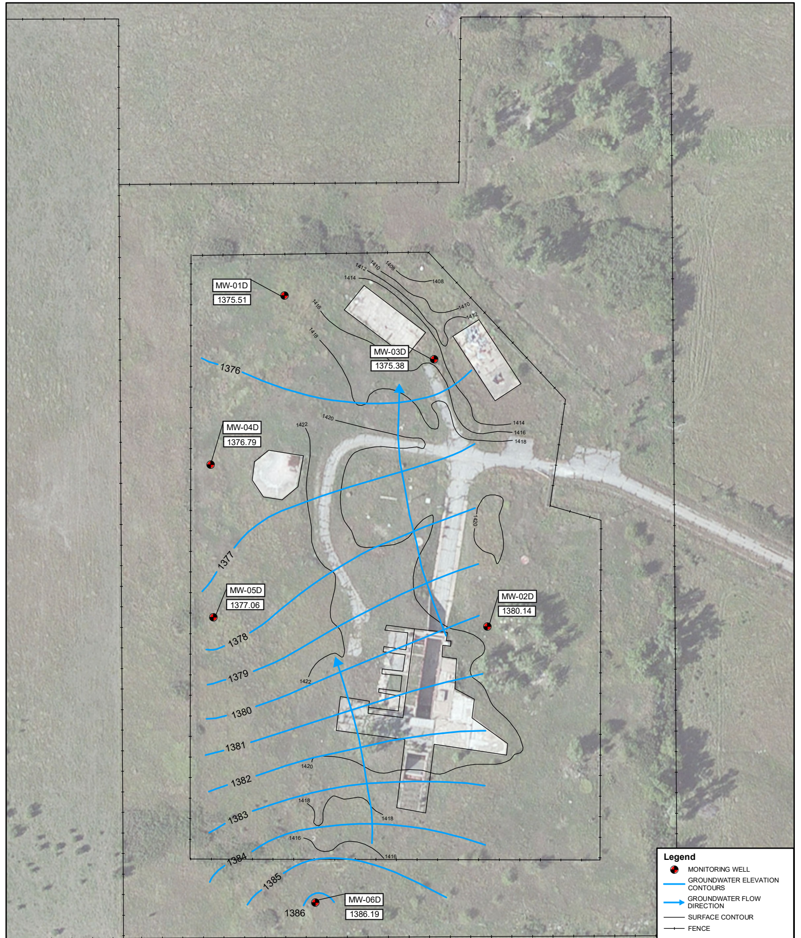
FIGURE 1 GROUNDWATER ELEVATION MAP DEEP MONITORING WELL LOCATIONS FORBES ATLAS S-5 ALLEN, KANSAS SEPTEMBER 21, 2015
