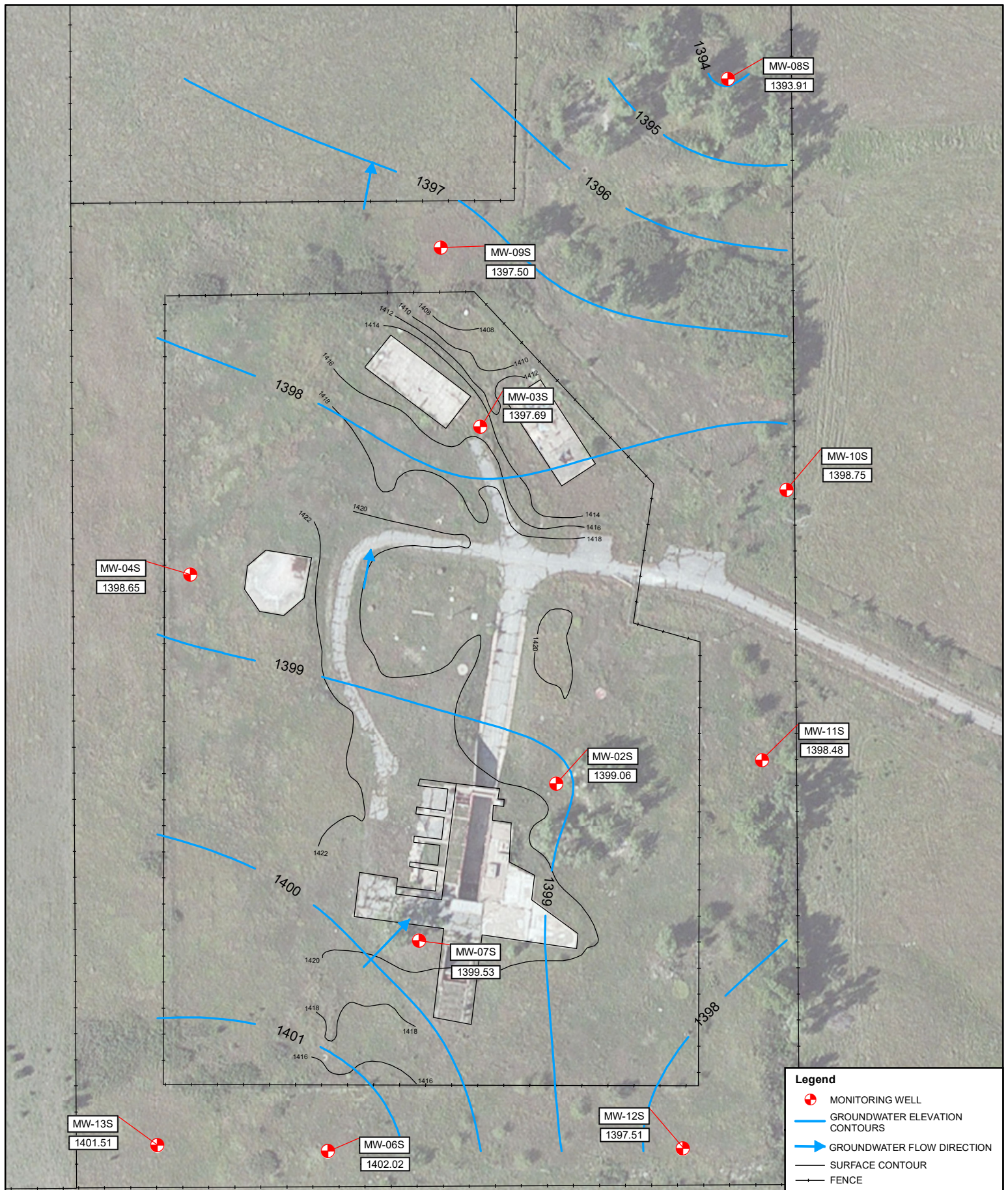
FIGURE 2 GROUNDWATER ELEVATION MAP SHALLOW MONITORING WELL LOCATIONS FORBES ATLAS S-5 ALLEN, KANSAS SEPTEMBER 12, 2016
