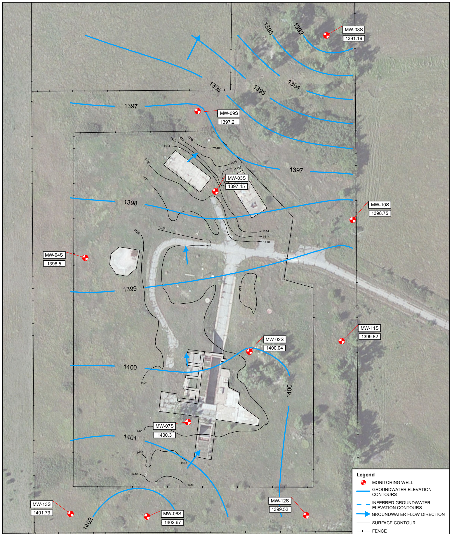
FIGURE 2 GROUNDWATER ELEVATION MAP SHALLOW MONITORING WELL LOCATIONS FORBES ATLAS S-5 ALLEN, KANSAS JUNE 27, 2016
