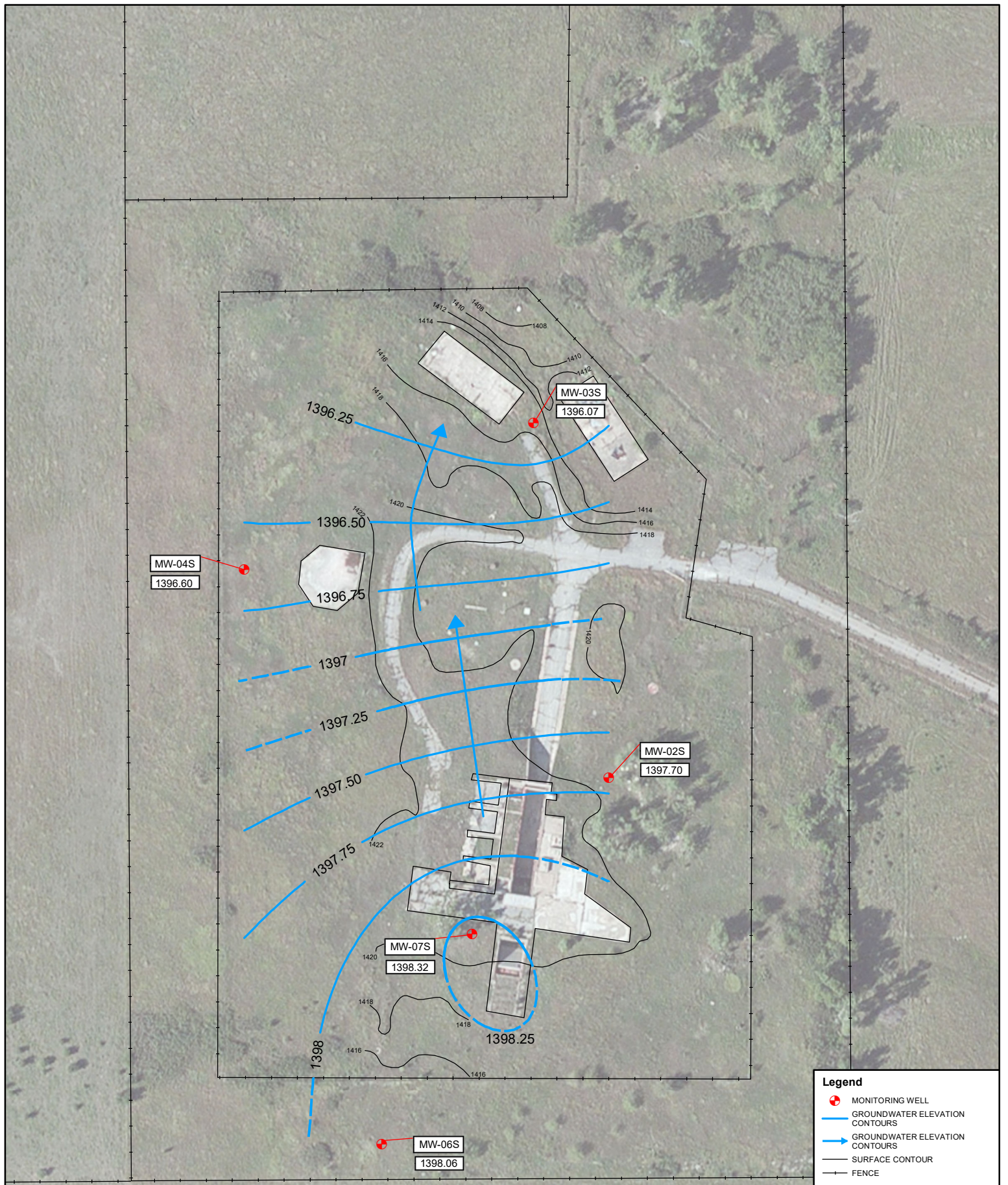
FIGURE 2 GROUNDWATER ELEVATION MAP SHALLOW MONITORING WELL LOCATIONS FORBES ATLAS S-5 ALLEN, KANSAS DECEMBER 14, 2015
