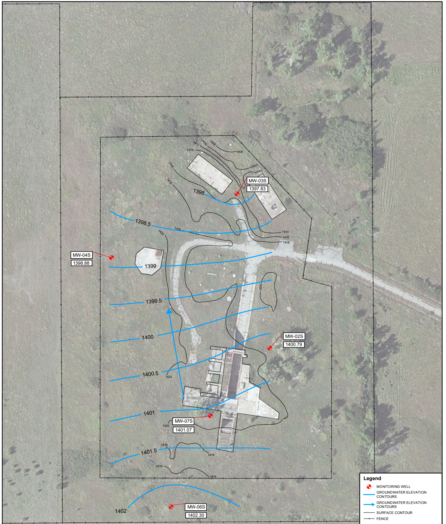
FIGURE 2 GROUNDWATER ELEVATION MAP SHALLOW MONITORING WELL LOCATIONS FORBES ATLAS S-5 ALLEN, KANSAS JULY 6, 2015
