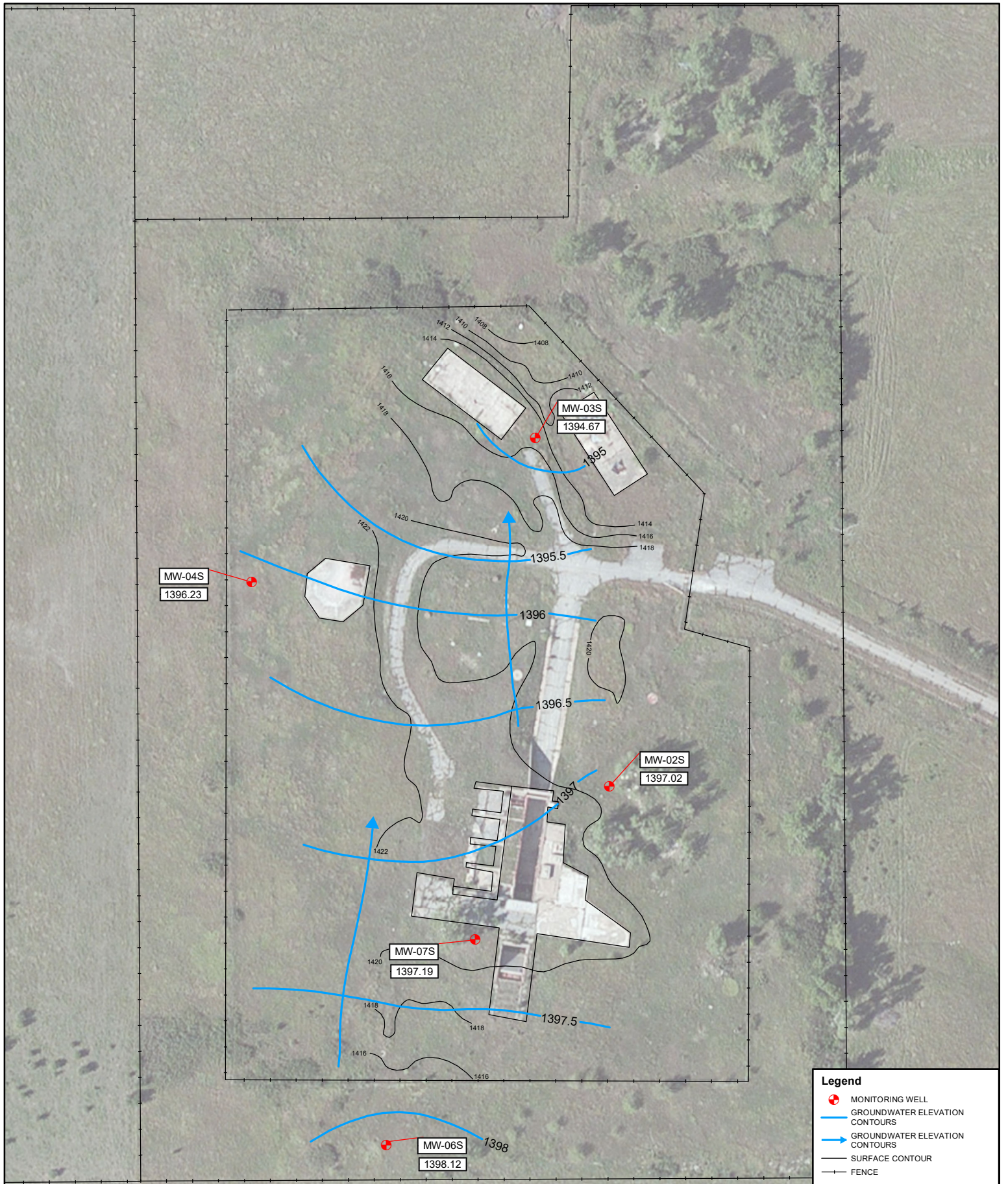
FIGURE 2 GROUNDWATER ELEVATION MAP SHALLOW MONITORING WELL LOCATIONS FORBES ATLAS S-5 ALLEN, KANSAS SEPTEMBER 21, 2015
