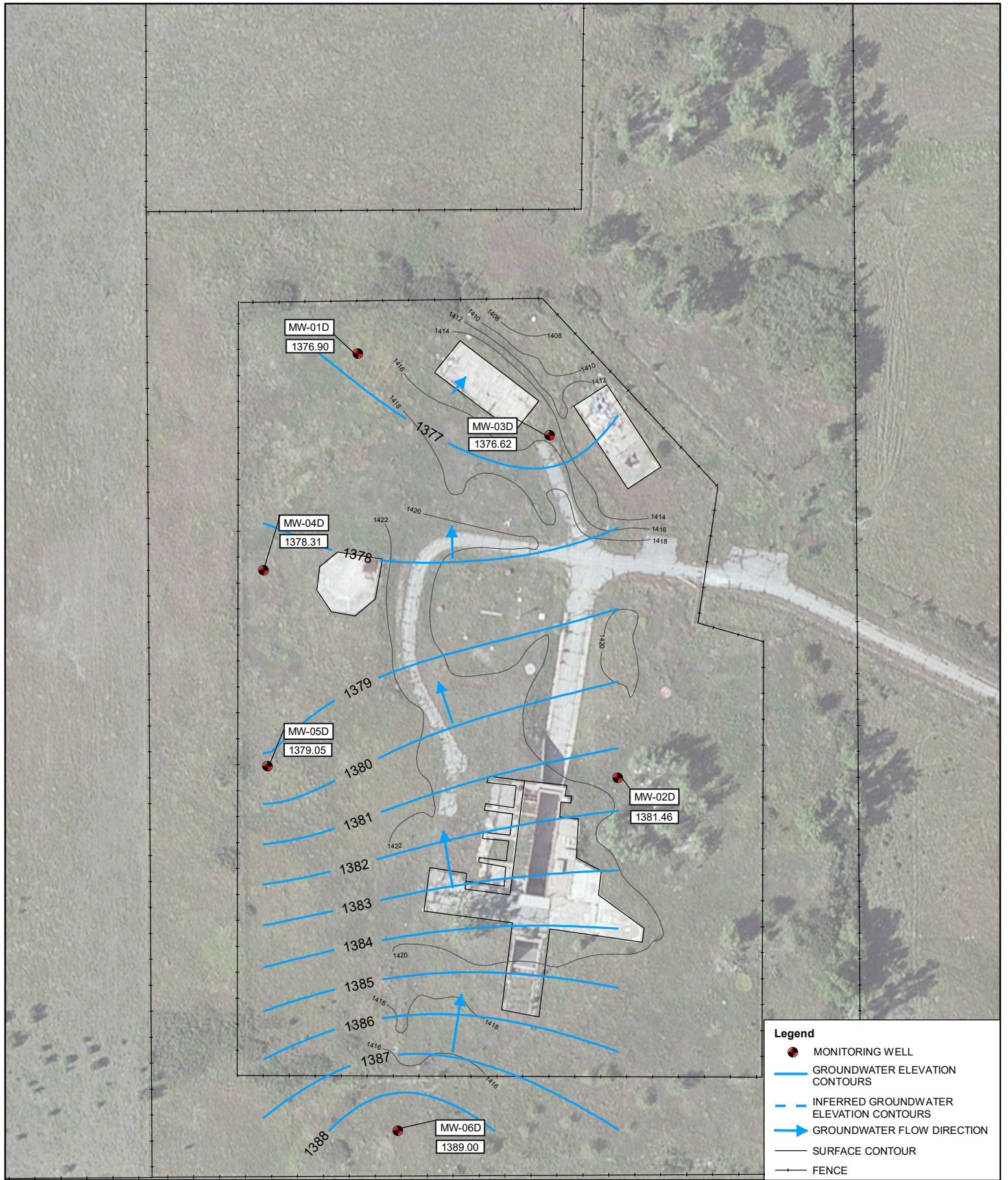
FIGURE 1 GROUNDWATER ELEVATION MAP DEEP MONITORING WELL LOCATIONS FORBES ATLAS S-5 ALLEN, KANSAS JUNE 27, 2016
