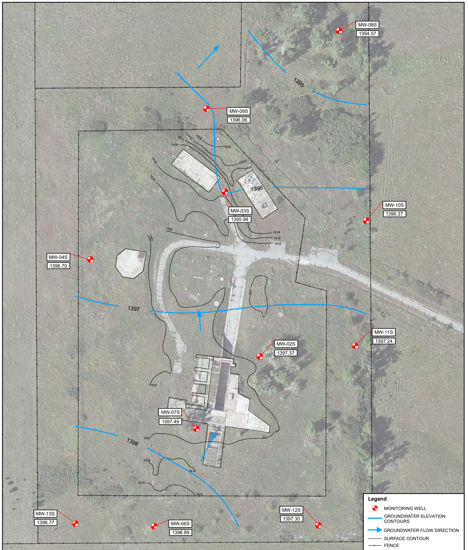
FIGURE 2 GROUNDWATER ELEVATION MAP SHALLOW MONITORING WELL LOCATIONS FORBES ATLAS S-5 ALLEN, KANSAS DECEMBER 12, 2016
