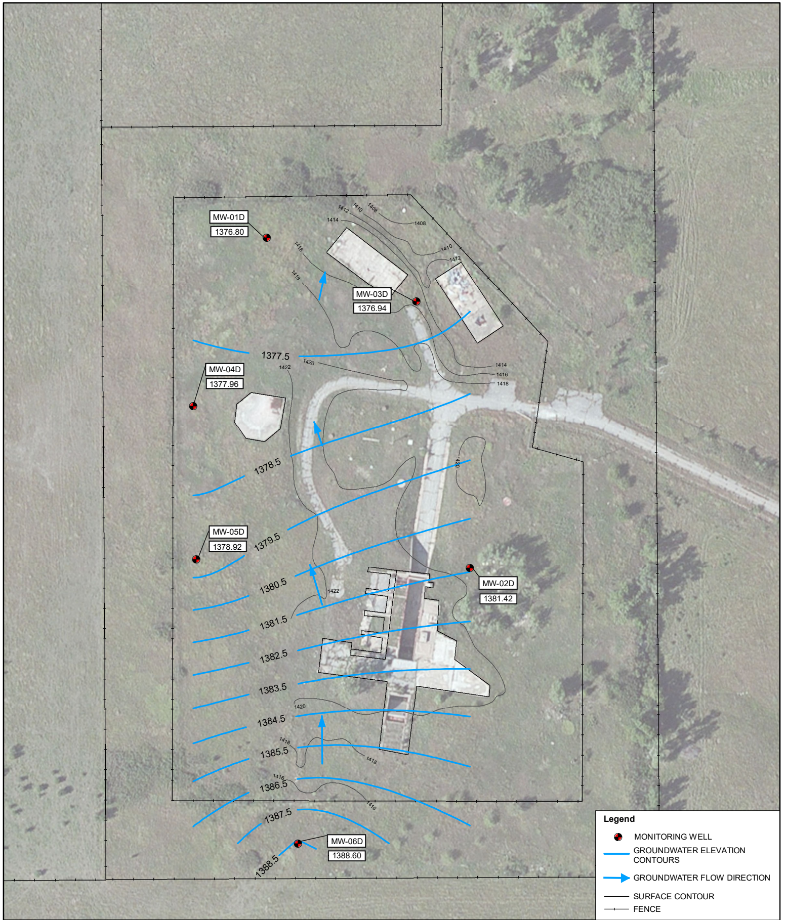
FIGURE 1 GROUNDWATER ELEVATION MAP DEEP MONITORING WELL LOCATIONS FORBES ATLAS S-5 ALLEN, KANSAS DECEMBER 12, 2016
