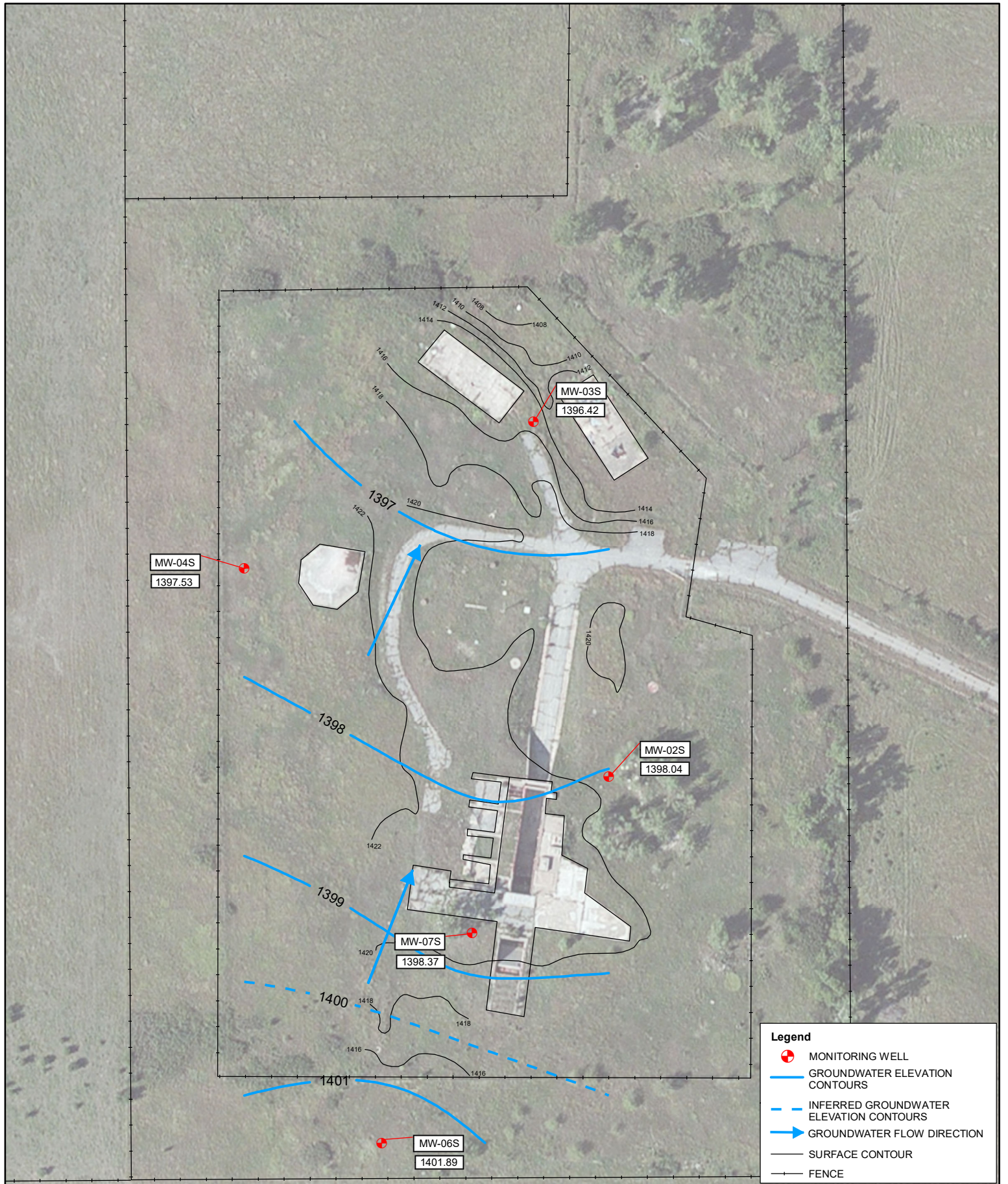
FIGURE 2 GROUNDWATER ELEVATION MAP SHALLOW MONITORING WELL LOCATIONS FORBES ATLAS S-5 ALLEN, KANSAS MARCH 7, 2016
