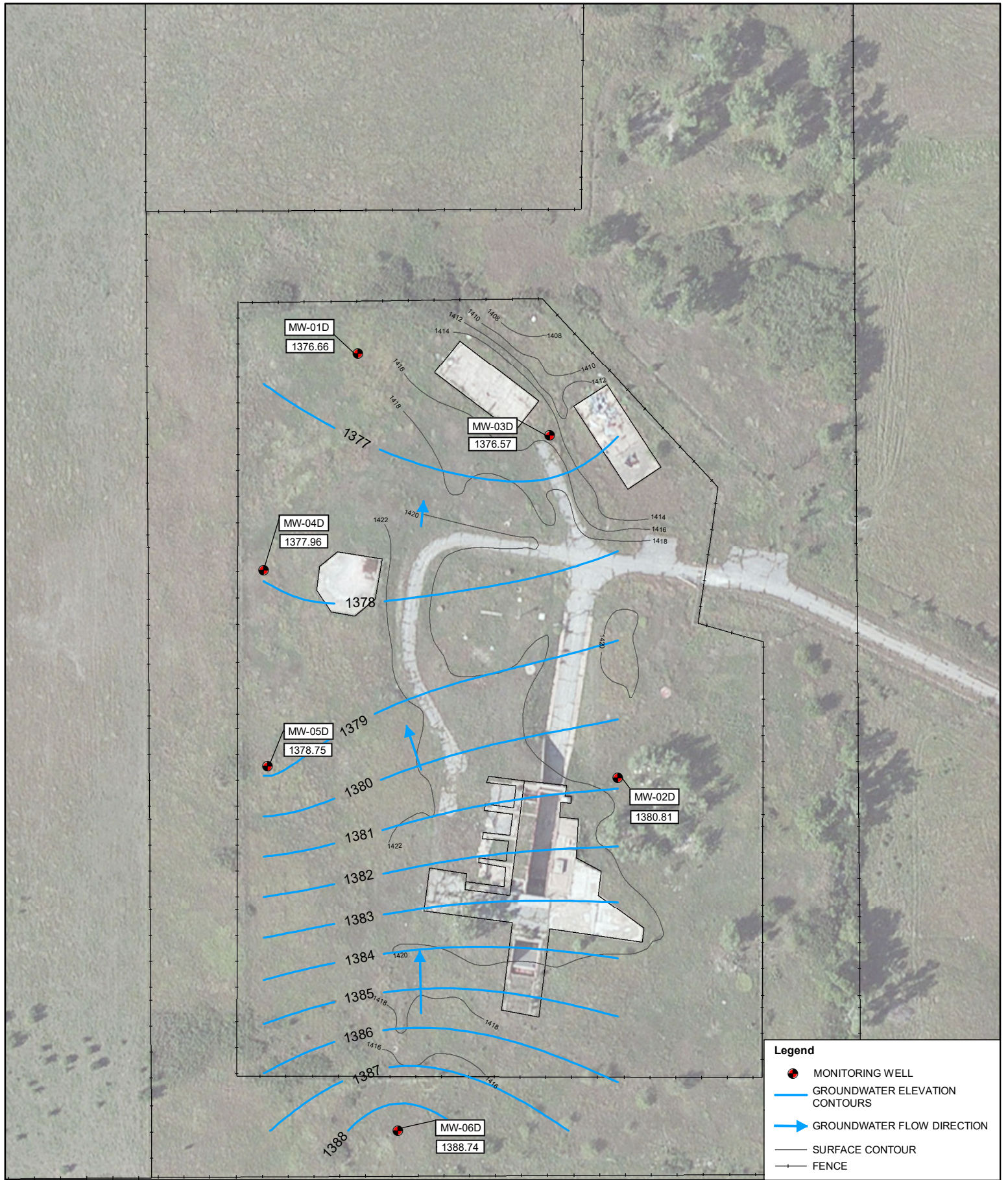
FIGURE 1 GROUNDWATER ELEVATION MAP DEEP MONITORING WELL LOCATIONS FORBES ATLAS S-5 ALLEN, KANSAS SEPTEMBER 12, 2016
